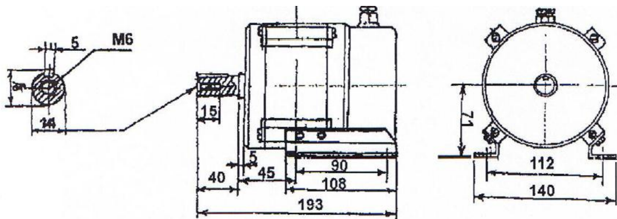
A Frame (Metric-71 frame) ó Foot Mount
