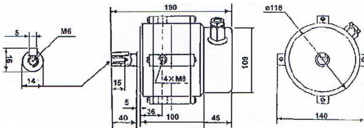
A Frame (Metric-71 frame) ó Pad Mount
