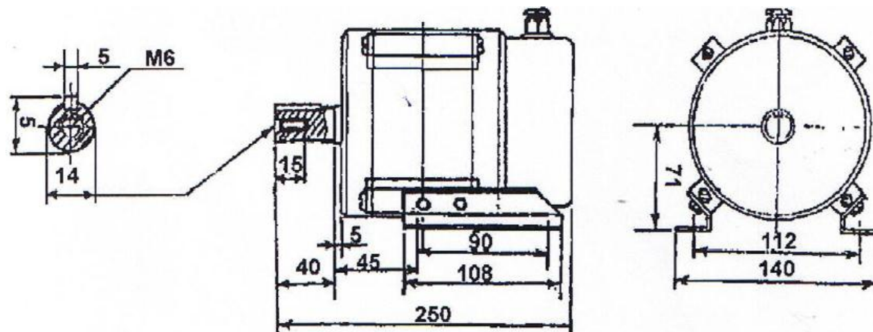
B Frame (Metric-71 Frame) \phi Foot Mount
